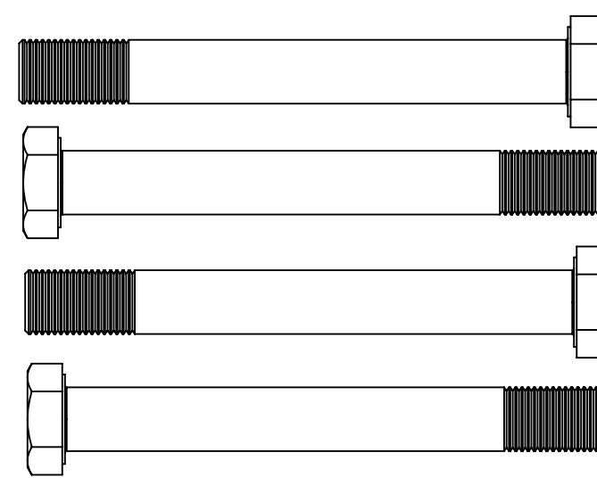
E00-2610 - 4 EA. AN6-31A 3/8 X 3-1/8 BOLT LANDING GEAR TO AIRFRAME
