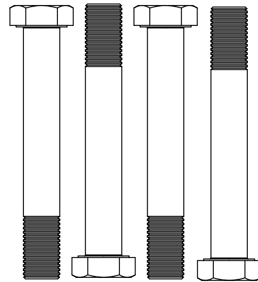
E00-2604 - 4 EA. AN6-24A 3/8 X 2-1/2 BOLT LANDING GEAR THRU SPRING TUBE
